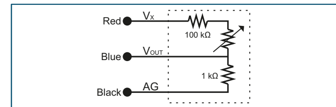
FoliarDB sensor-cable connector Leaf wetness sensor
